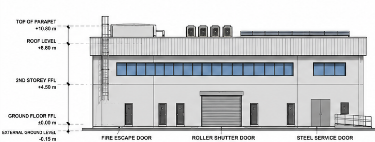
SOUTH ELEVATION (REAR)
